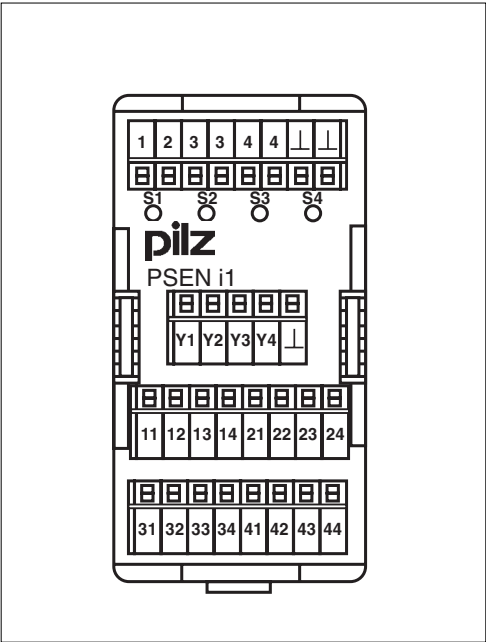
Terminal configuration
