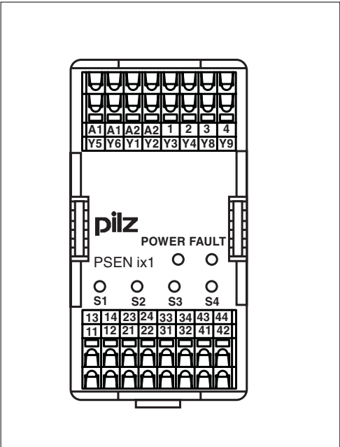
Terminal configuration
