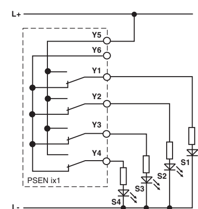
LED lights when the safety gate is closed
